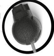
Freakshow Symmetric
